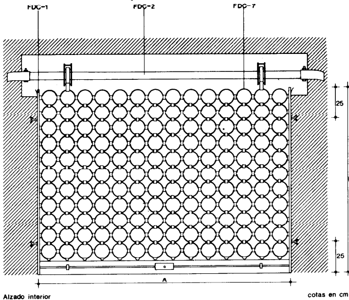
Alzado interior
